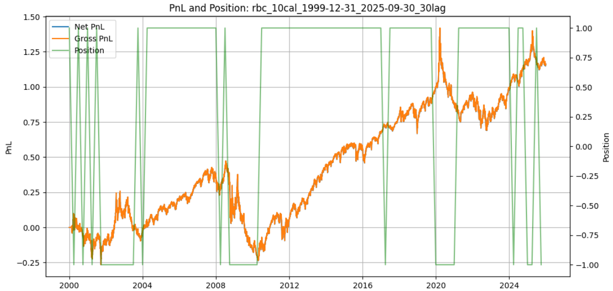
Figure 6: PnL and positions for RBC 10y 1999-12-31_2025-09-30 30lag MR strategy
