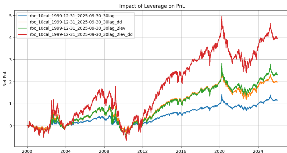
Figure 11: PnL with doubling down and 2x leverage of RBC 10y 1999-12-31_2025-09-30 30b lag strategy
